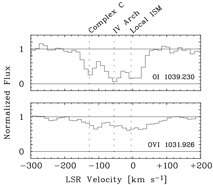
Figure 1. Interstellar absorption of neutral oxygen (O I) and highly-ionized oxygen (O VI) in the direction of the quasar PG 1259+593 ( l = 120.6 , b = +58.1 , z_{\text{em}} = 0.478 ). The O I absorption shows two Galactic halo components at -128 \text{ km s}^{-1} (high-velocity cloud Complex C) and at -55 \text{ km s}^{-1} (intermediate-velocity cloud IV Arch), while local ISM absorption is seen at -5 \text{ km s}^{-1} . These three main velocity components are marked with dotted lines. Also the O VI absorption extends to high negative velocities, possibly arising in the interface regions between the neutral HVC gas (as sampled by O I) and a surrounding hot medium - the Galactic Corona (see also Fox et al. 2003).
